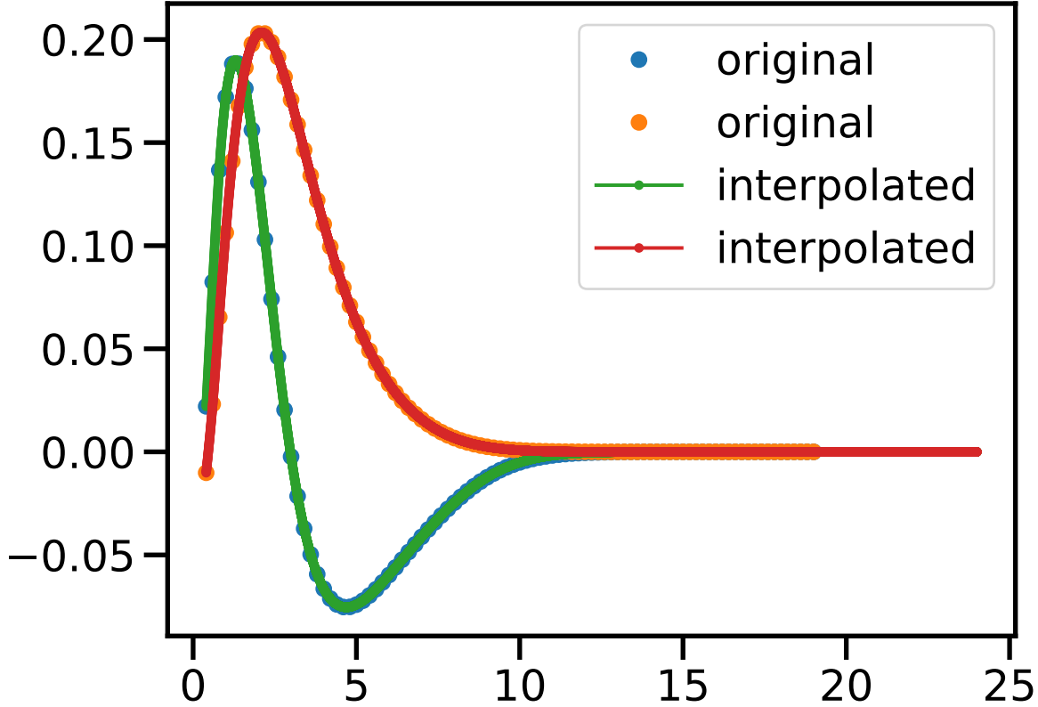
Hamiltonian Interpolation Before Training (14, 14, 1, 2)
